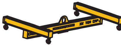
OPTION B Adjustable Bail Used when load-leveling capability is required along length of load.
